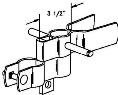
DROP ROD FORK AND GUIDE
