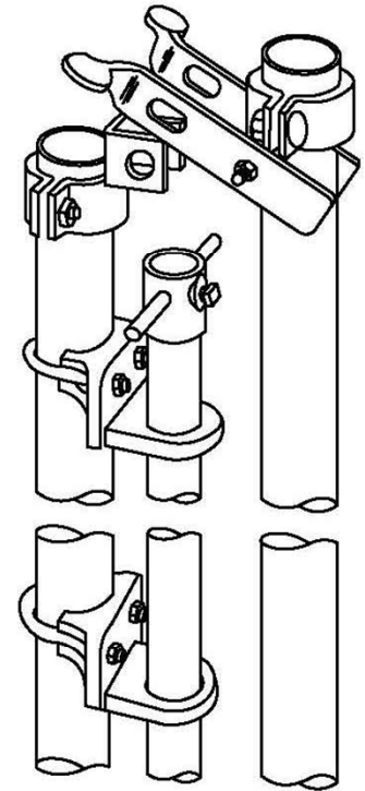
INDUSTRIAL CENTER LOCKING GATE NO. 6448 1 5/8" OR 2"
